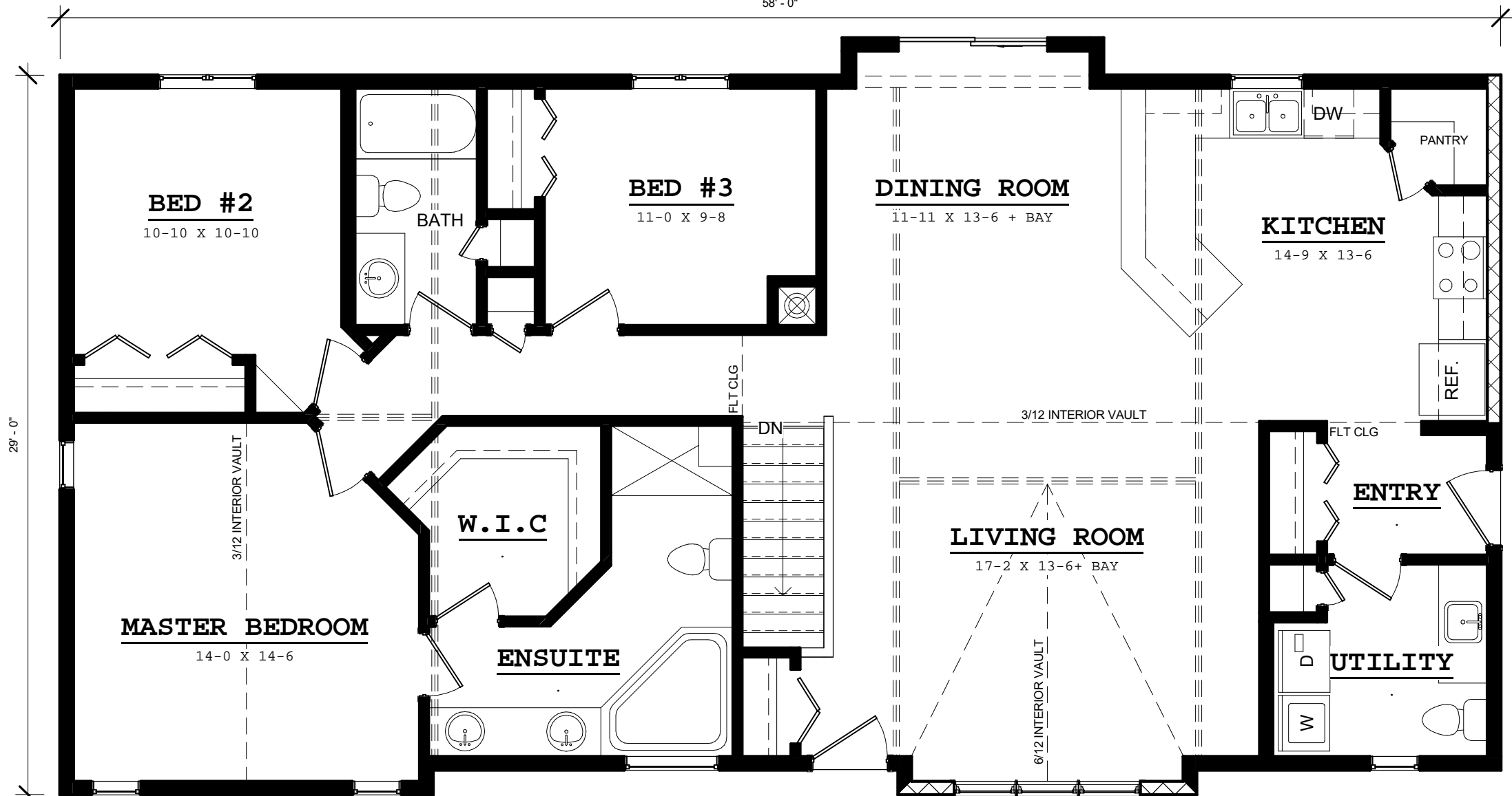
MAIN FLOOR 1669 SQUARE FEET
