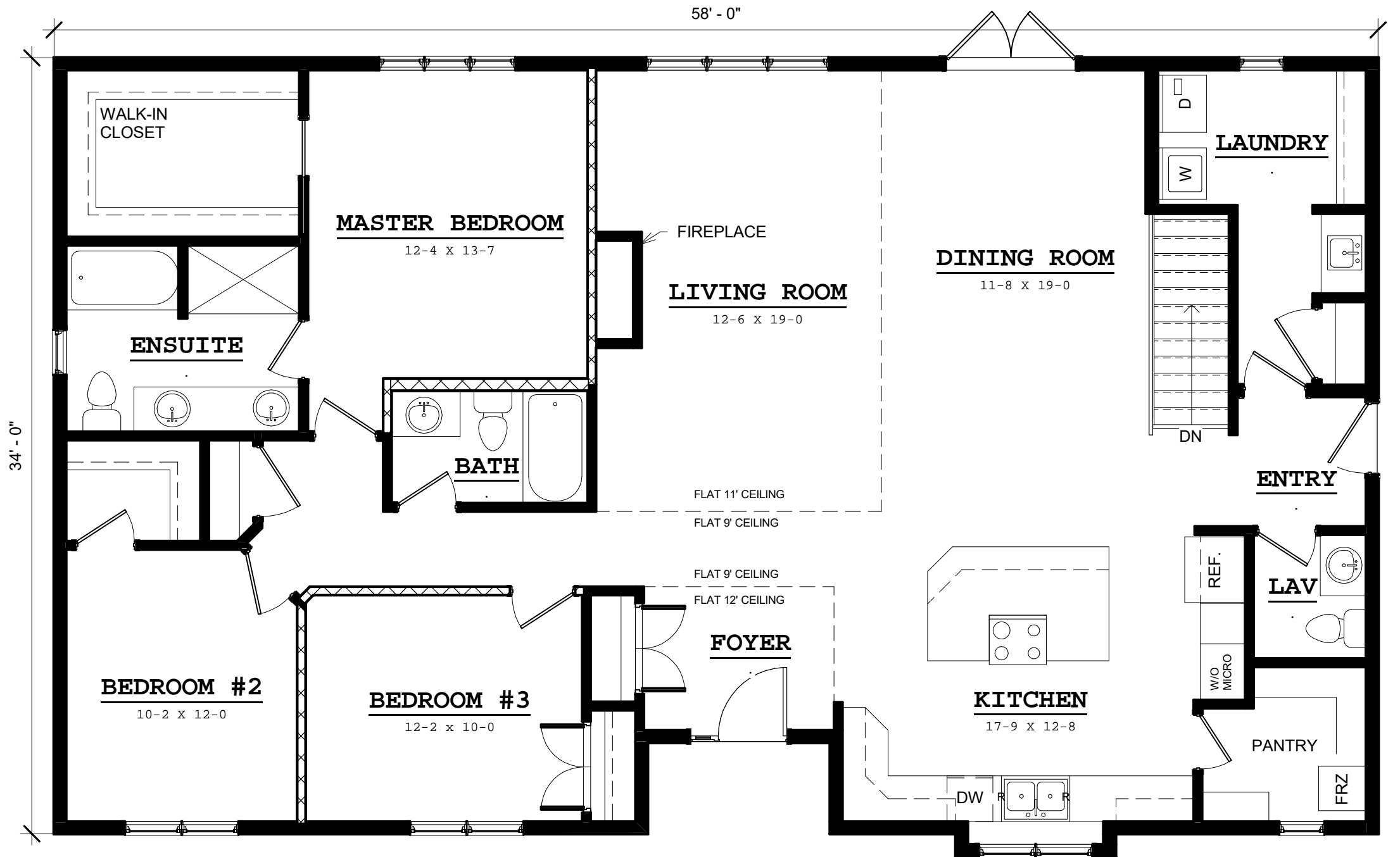
MAIN FLOOR 1940 SQUARE FEET
