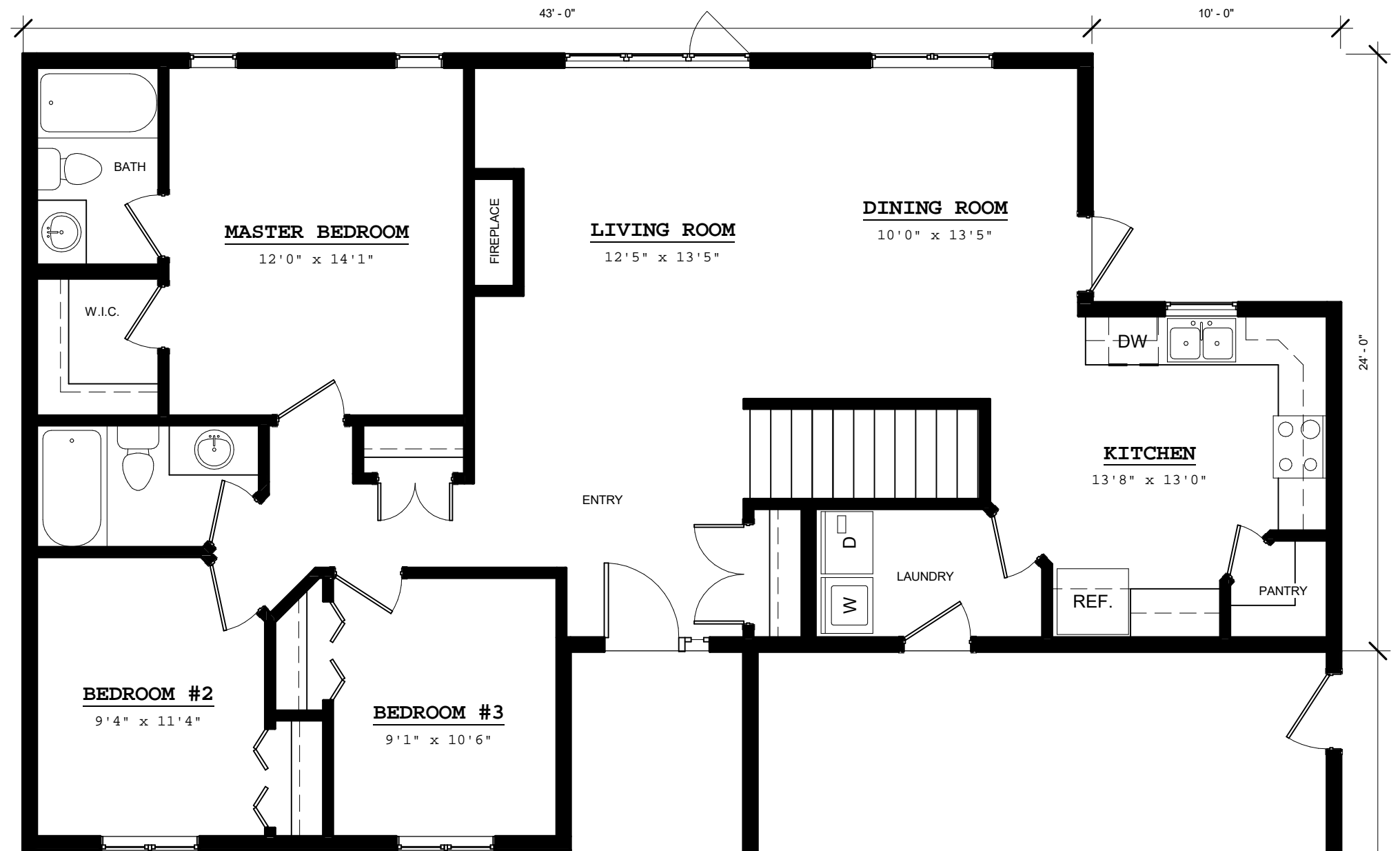
MAIN FLOOR 1348 SQUARE FEET
