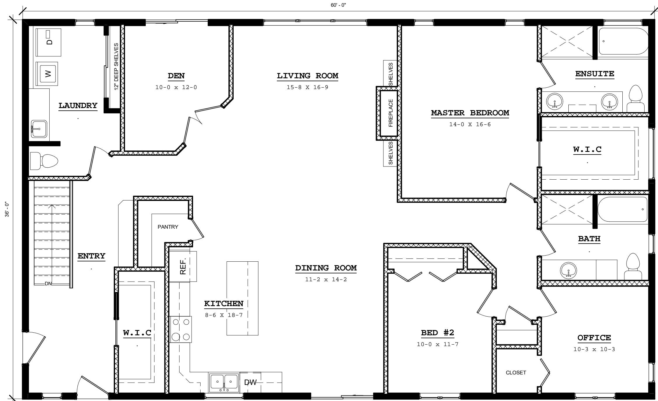
MAIN FLOOR PLAN 2160 SQUARE FEET
